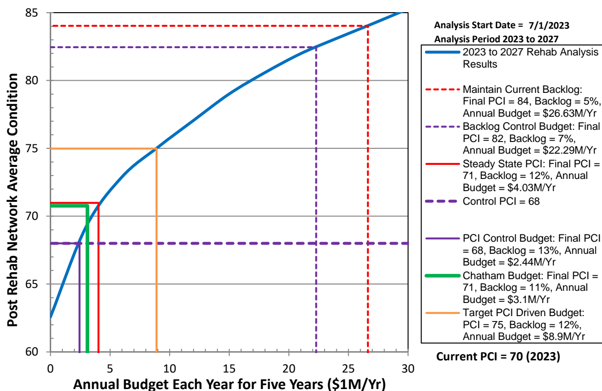
Figure 17 – Five-year Post Rehab Network PCI Analysis Results
