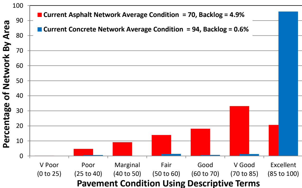
Figure 15: Current Pavement Condition By Pavement Type
