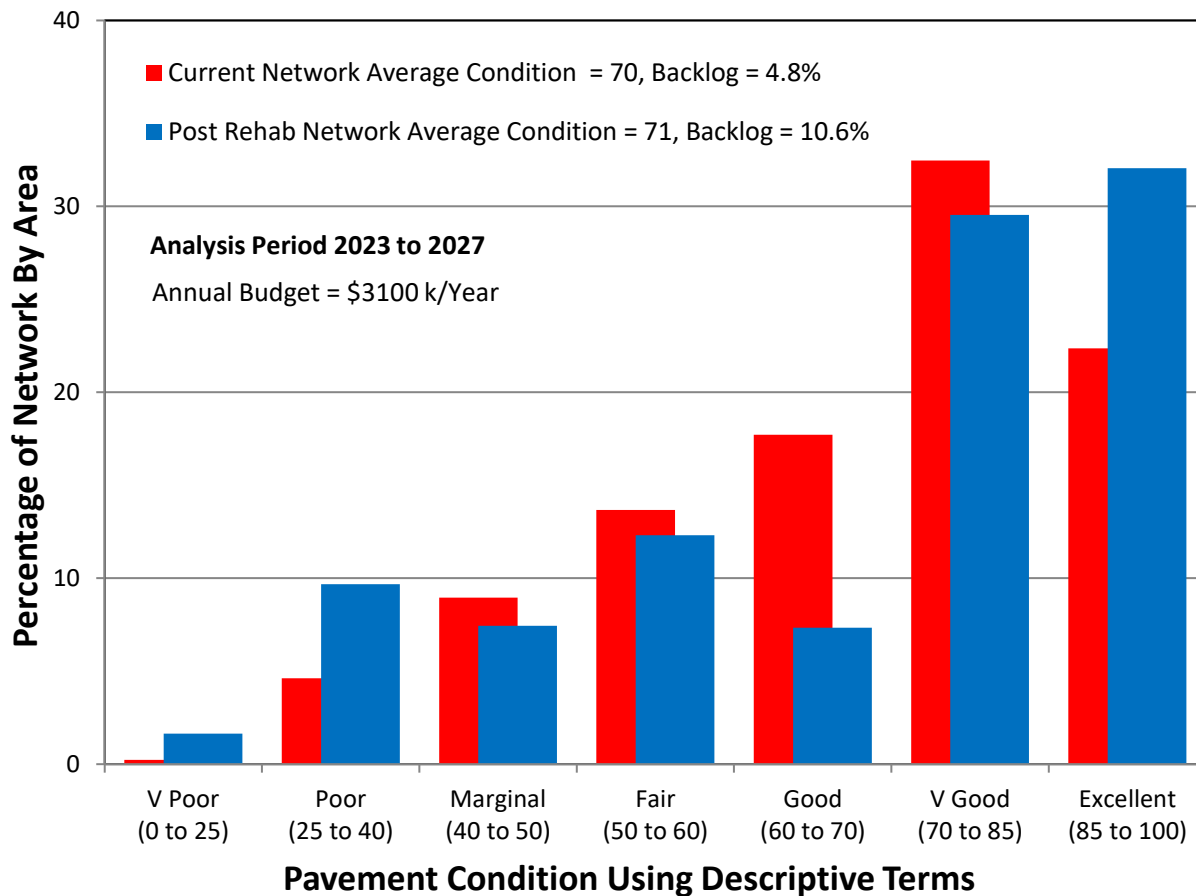
Figure 20 – Comparison of Pavement Condition Outcome of Two Potential Budgets over Five Years
