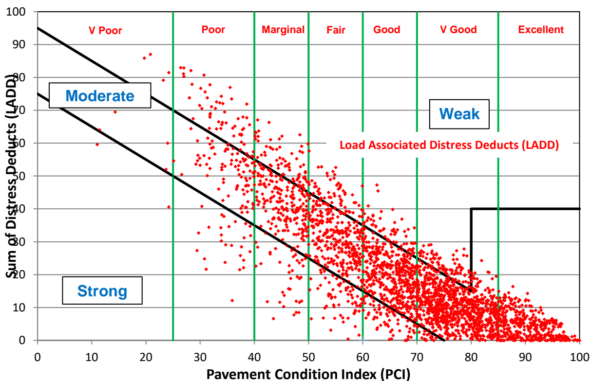
Figure 16 - LAD compared to PCI
