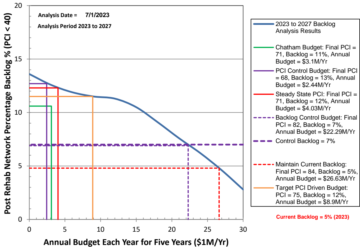
Figure 18 – Five-year Post Rehab Network Backlog Results
