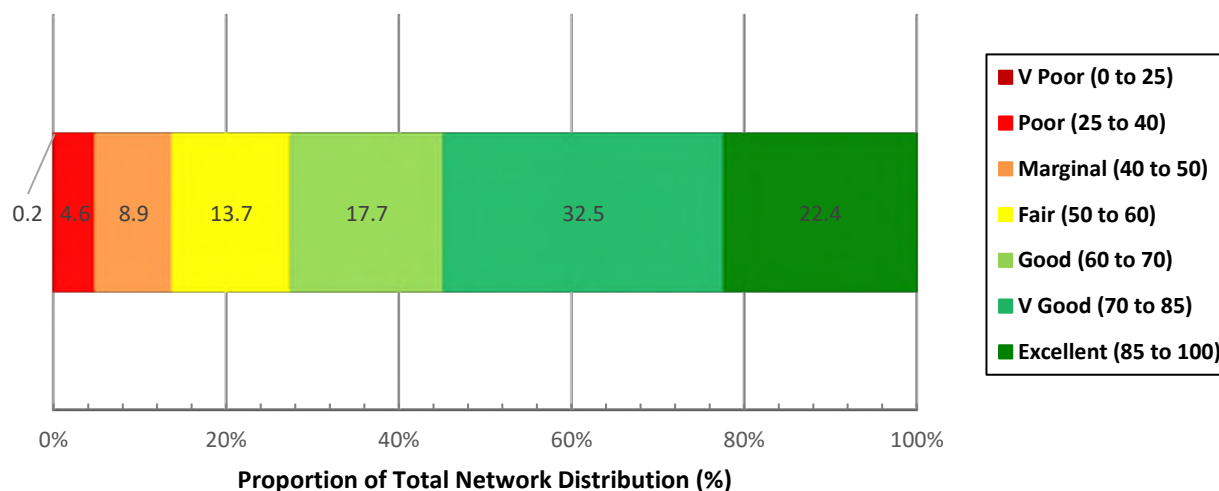
Figure 2 - Distribution of the County's Pavement System on a Condition Scale
